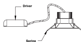
Connect power and fix the fixture into Ceiling
